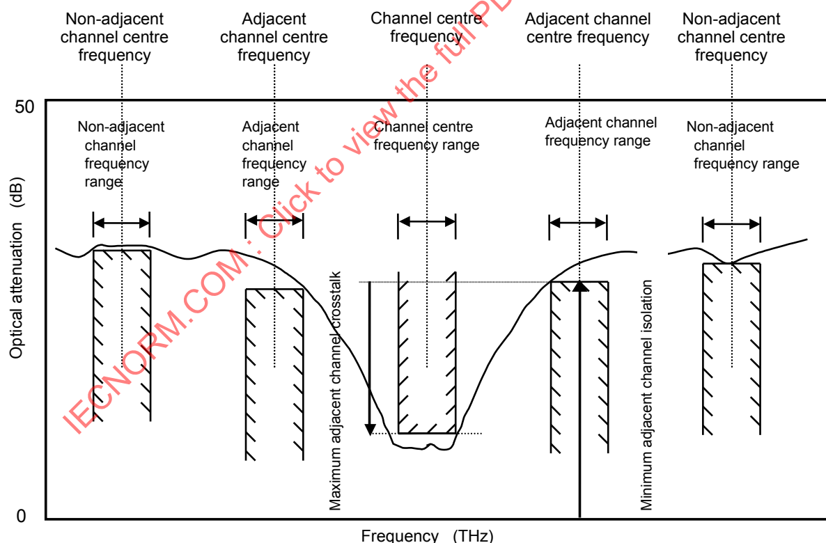
Figure 11 – Minimum adjacent channel isolation
