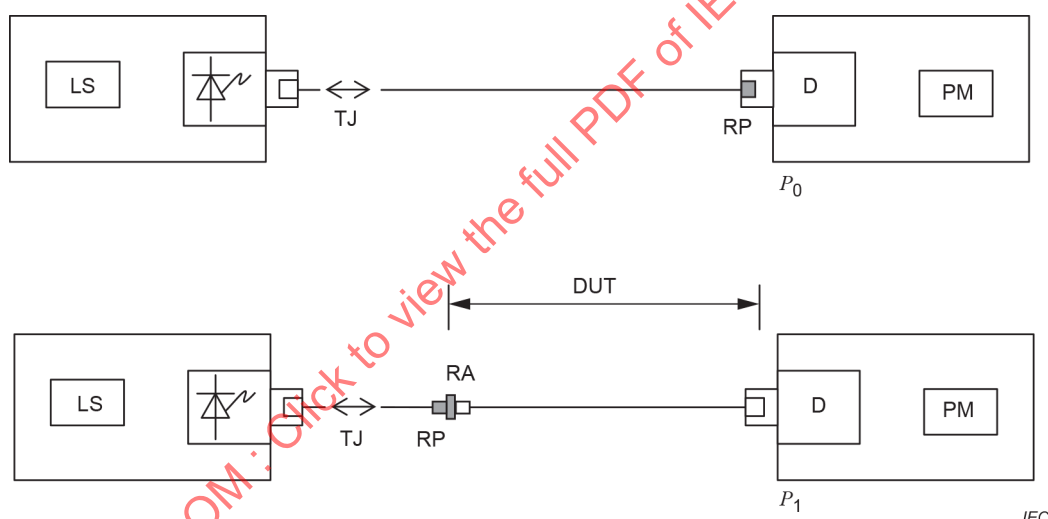
Figure 4 – Insertion method (C2B) – Type 5 and type 6 DUT
