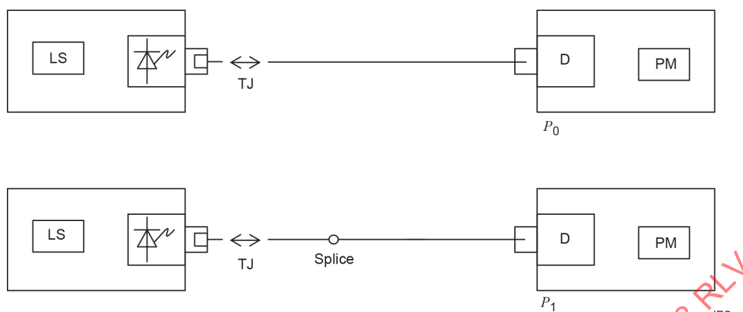
Figure 3 – Insertion method (C4A) – Type 2 DUT
