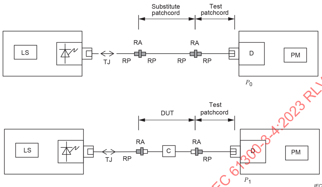
Figure 2 – Substitution method – Type 4, type 7, and type 8 DUT
