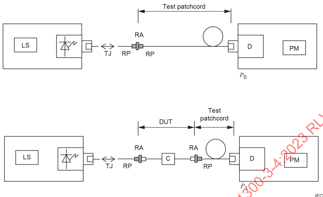
Figure 5 – Insertion method (C3C) – Type 4, type 5, type 7 and type 8 DUT
