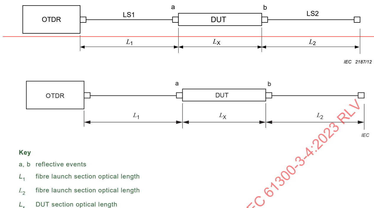
Figure 8 – Method 2 – Two launch sections
