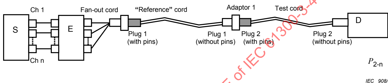
Figure 9 – Test cord measurement (2) – Method 2
