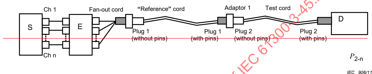
Figure 7 – Test cord measurement (1) – Method 2
