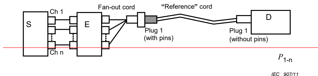
Figure 8 — “Reference” cord measurement (2) — Method 2
