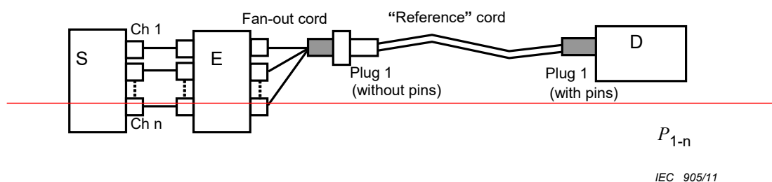
Figure 6 – “Reference” cord measurement (1) – Method 2
