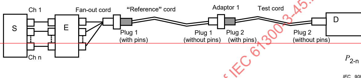
Figure 9 — Test cord measurement (2) — Method 2
