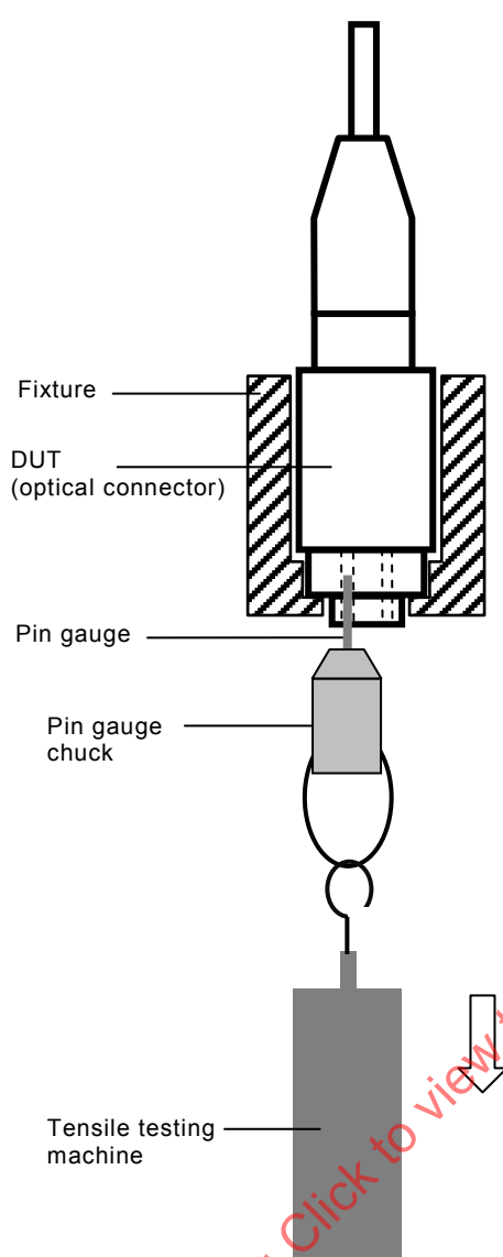
Figure 4a – Measurement for single hole
