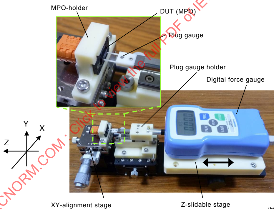
Figure A.1 – Measurement system
