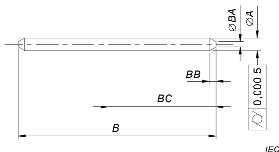
Figure 1 – Broche calibrée
