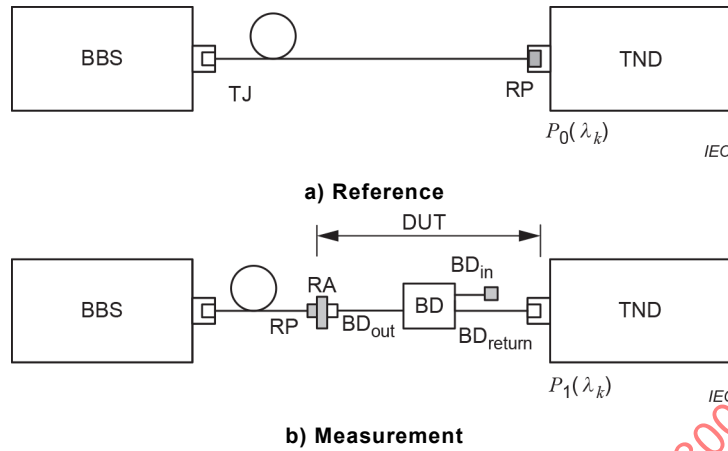
Figure 4 – Method A2, attenuation and return loss, reference branching device measurement set-up
