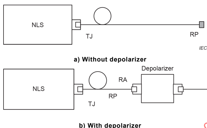
Figure 8 – Method B, tuneable narrowband light source with and without depolarizer
