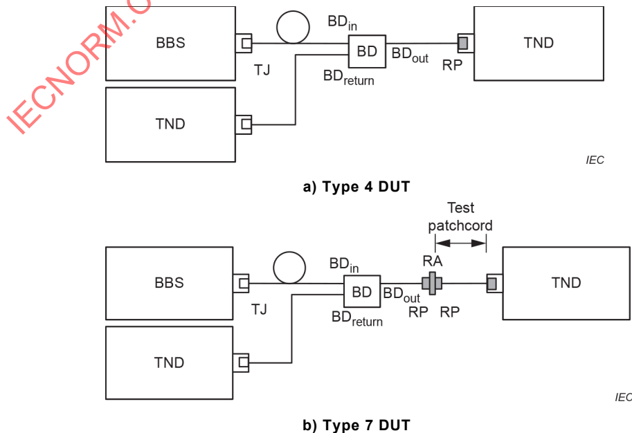
Figure 5 – Method A2, attenuation and return loss, reference measurement set-up
