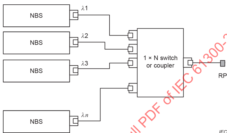
Figure 9 – Method C, multiple fixed narrowband sources set-up
