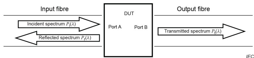
Figure 1 – Generic explanation of attenuation and return loss
