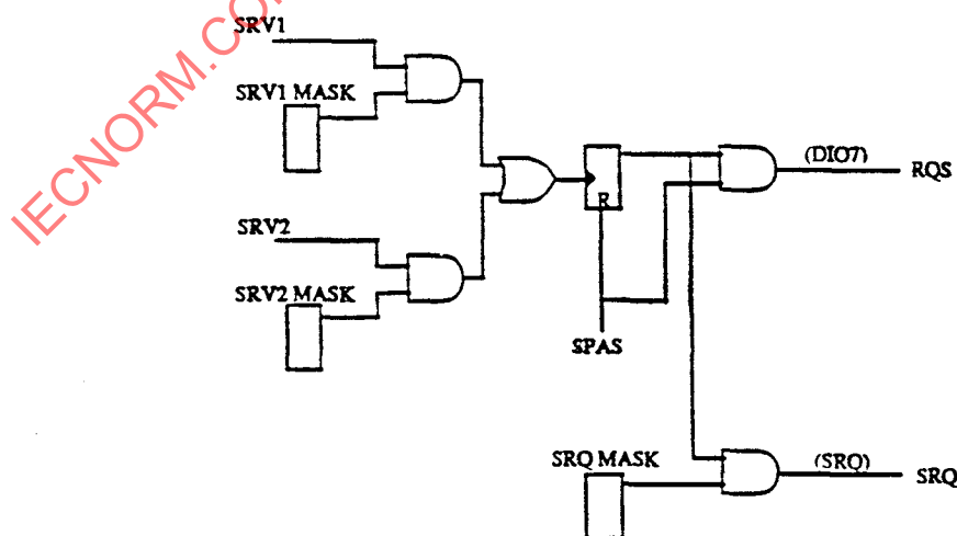
Figure 1 – Example of implementation of the serial poll feature in a NIM/625 module
