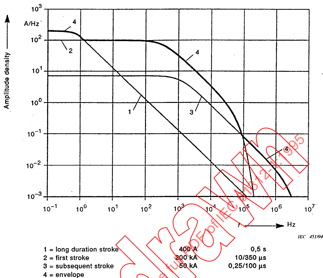
Figure B.5 – Amplitude density of the lightning current according to protection level I
