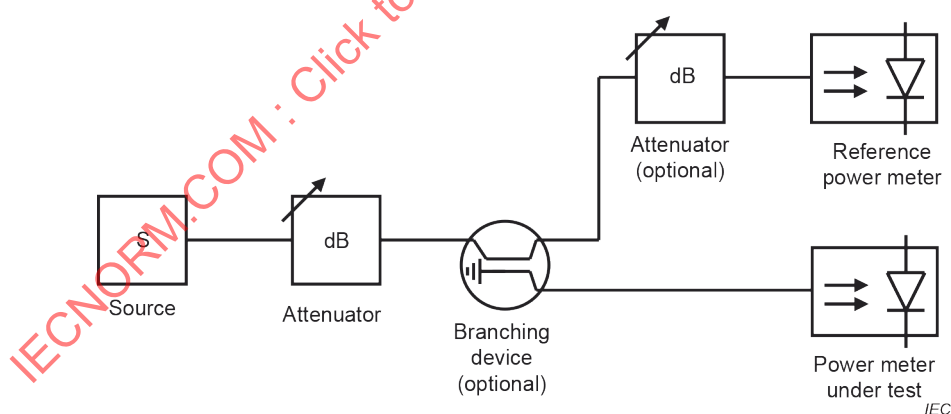
Figure 10 – Measurement setup for nonlinearity calibration by comparison
