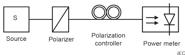
Figure 8 – Measurement setup of polarization dependent response
