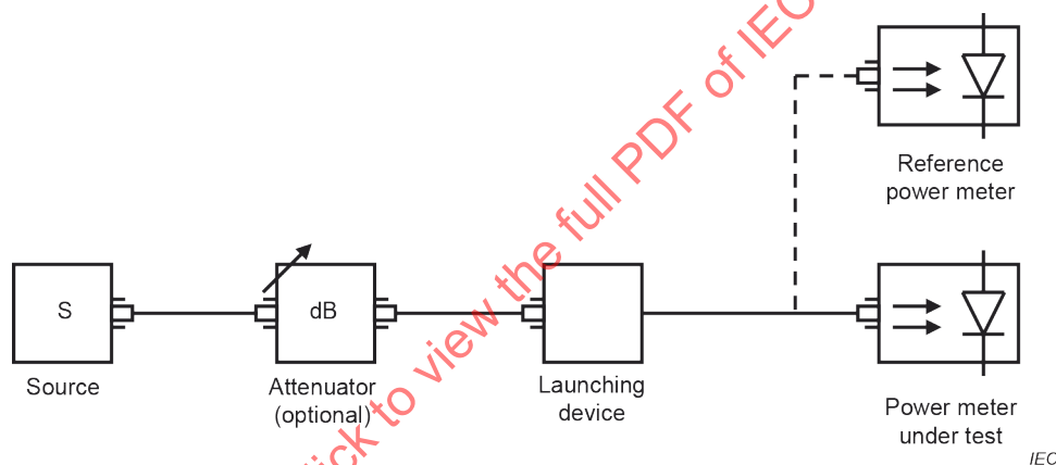
Figure 3 – Measurement setup for sequential, fibre-based calibration
