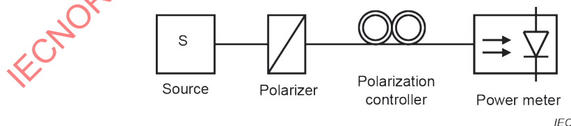
Figure 8 – Measurement setup of polarization dependent response
