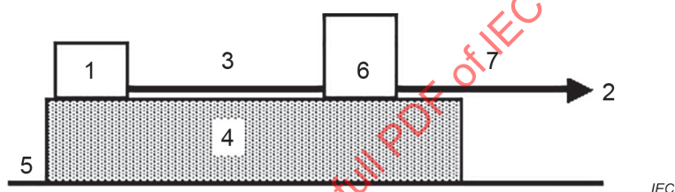
Figure CC.1 – Example of the configuration of a temperature transducer with sensor and signal conditioning in the same housing
