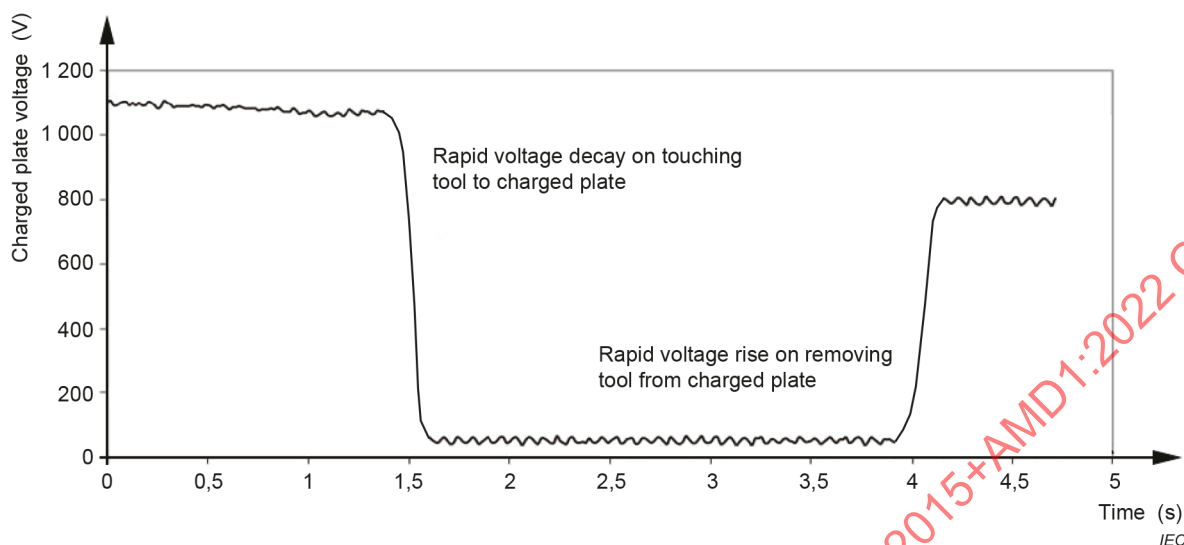
Figure 5 – Examples of decay waveforms when testing tools
