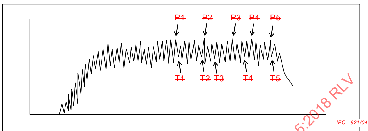
Figure 2a — Positive polarity body voltage recording
