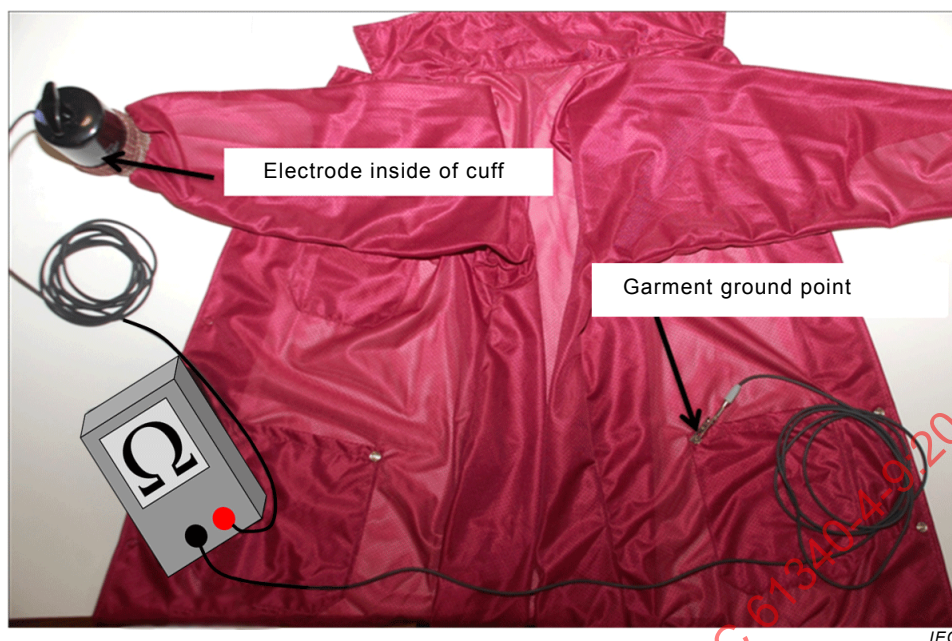
Figure 8 – Test set-up – Resistance point-to-groundable point (cuff-to-groundable-point procedure with insulative sleeve inserts)
