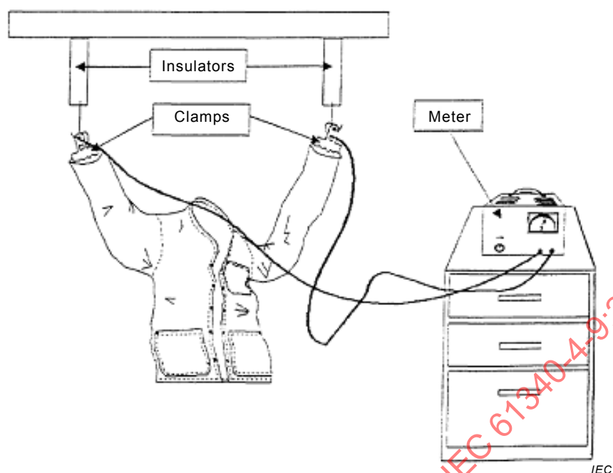
Figure 6 – Test set-up – Resistance point-to-point (hanging clamp sleeve-to-sleeve procedure)
