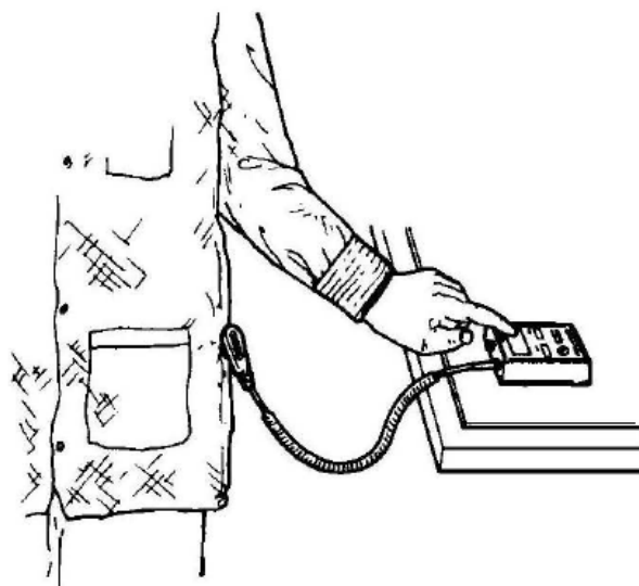
Figure 12 – Test set-up – Groundable static control garment system resistance (groundable garment in combination with a person using an integrated tester)
