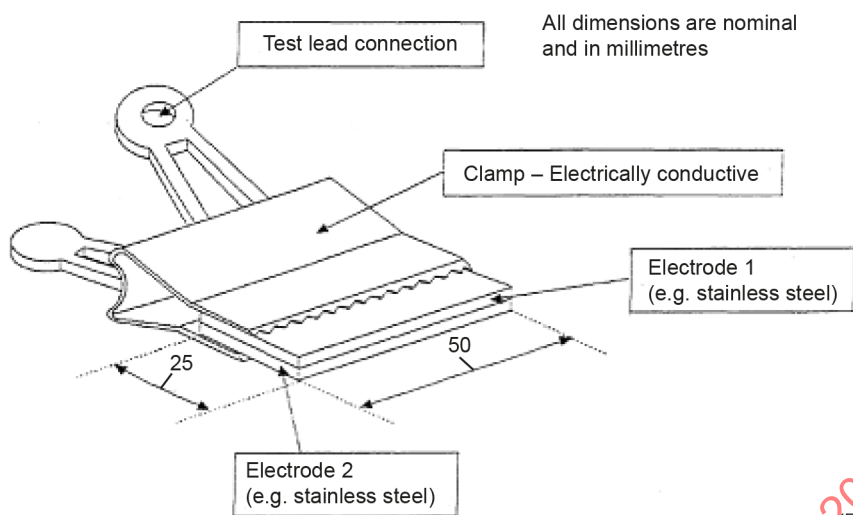
Figure 7 – Clamps or electrodes for hanging garment test
