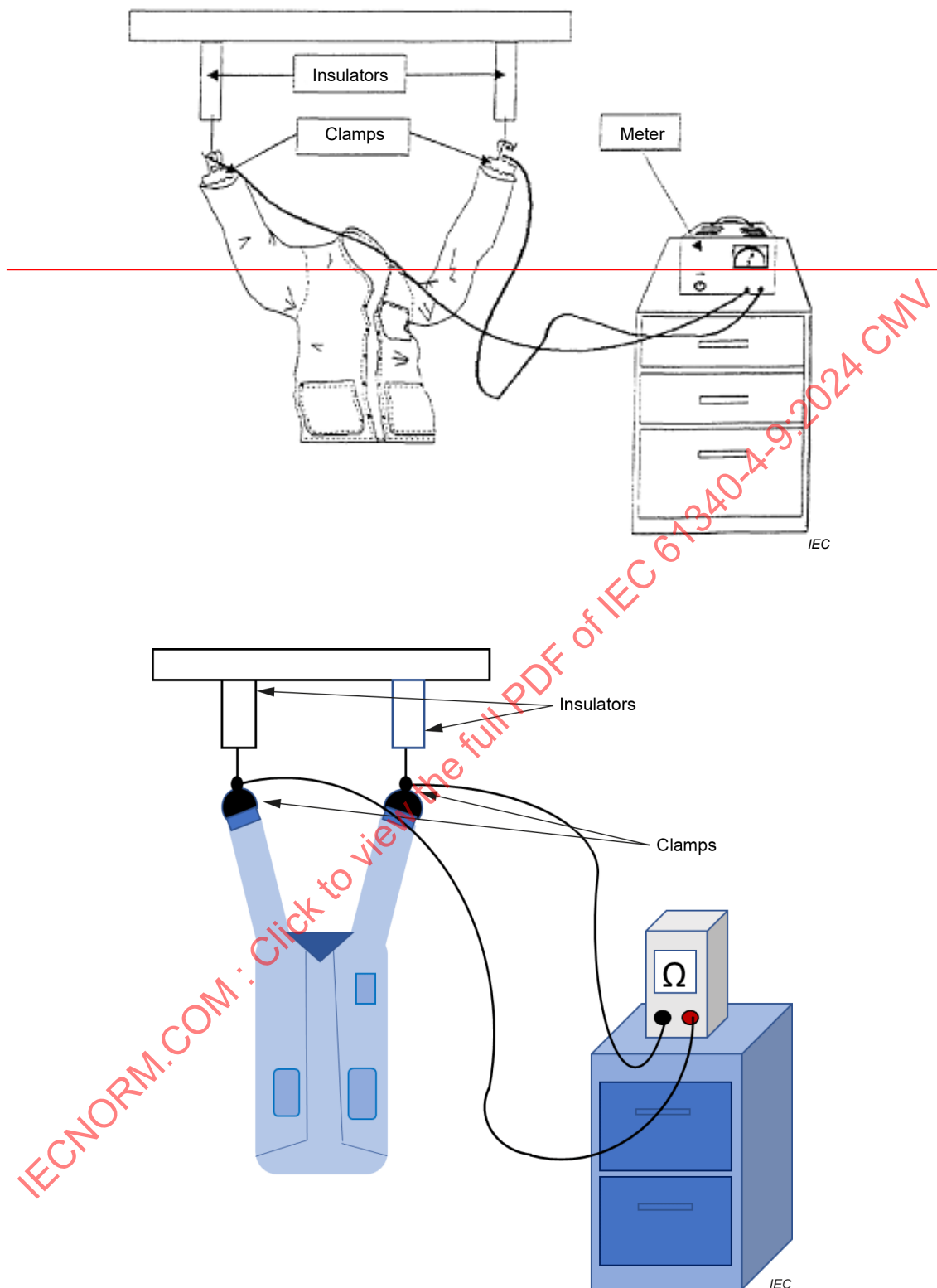
Figure 6 – Test set-up – Resistance point-to-point (hanging clamp sleeve-to-sleeve procedure)
