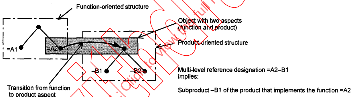
Figure 27 - Transition from function to product aspect
