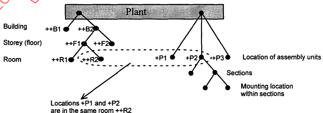
Figure 23 - Location-oriented structures of the plant
