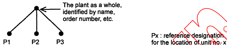
Figure 21 - Location-oriented structure of a plant
