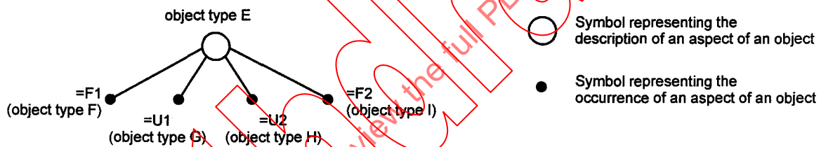
Figure 16 - Function-oriented structure of object type E
