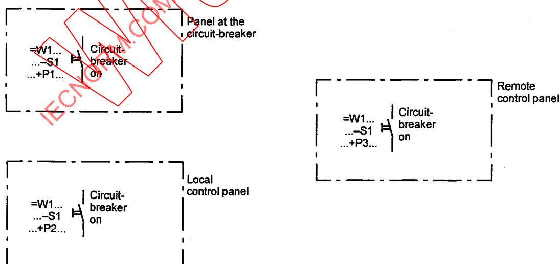
Figure 33 - Examples of reference designation groups
