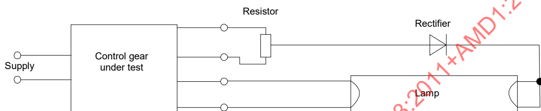
Figure 4a – Testing the first direction of the rectifying effect
