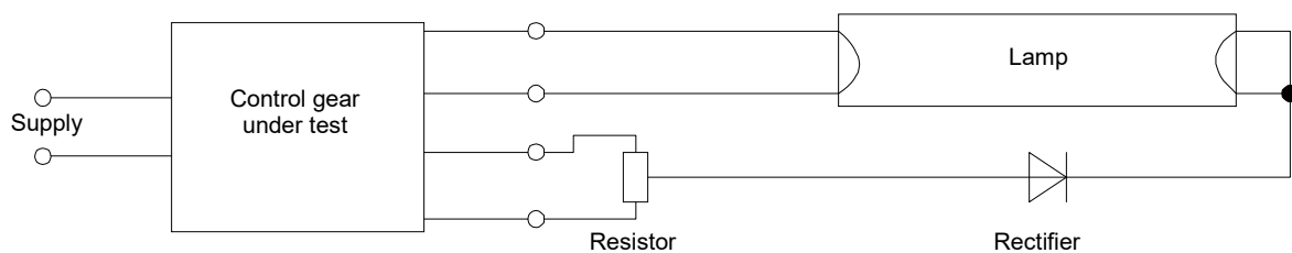
Figure 4a – Testing the first direction of the rectifying effect
