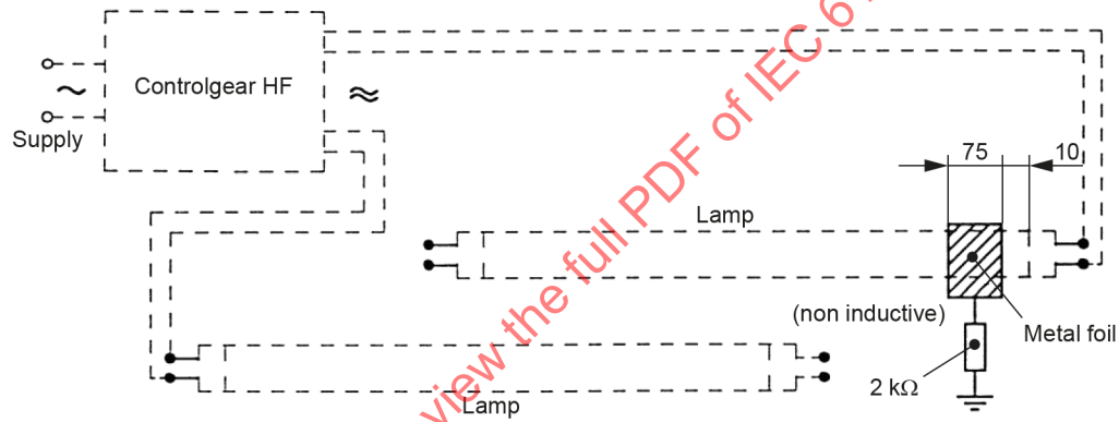
a) Test arrangement for bar-shaped tubular fluorescent lamps
