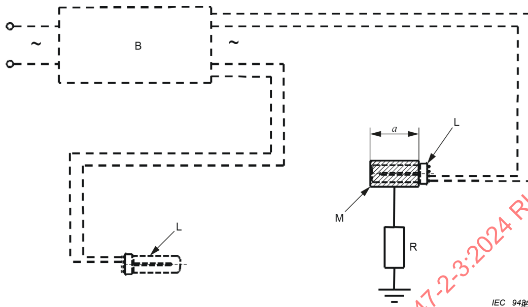
b) Test arrangement for lamps with ILCOS FSD (H)
