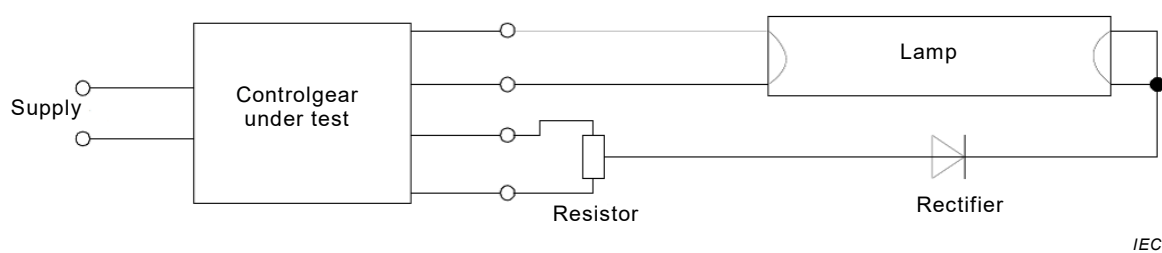
a) Testing the first direction of the rectifying effect
