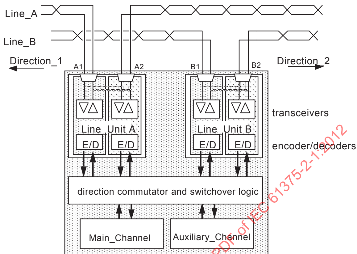
Figure 20 – Node with redundant Line Units
