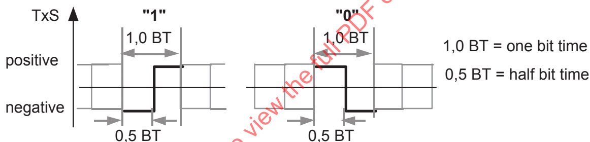
Figure 30 – Bit encoding
