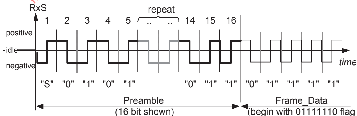
Figure 31 – Preamble
