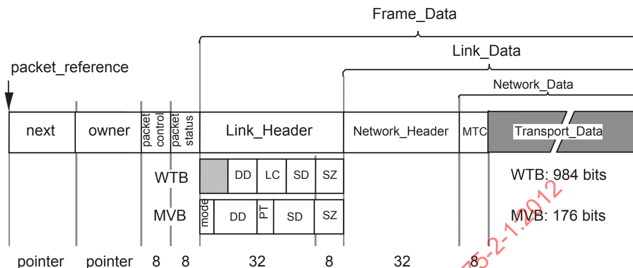
Figure 117 – Packet format
