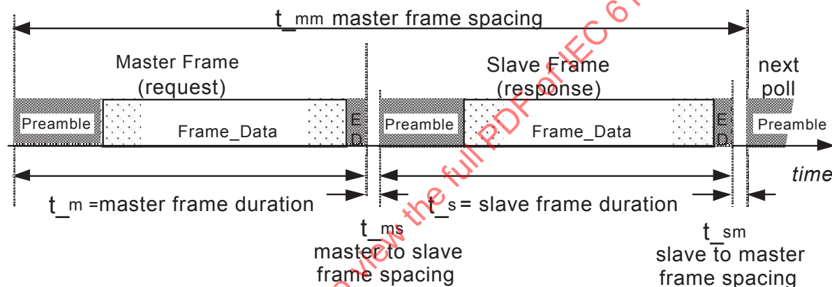
Figure 38 – Telegram timing
