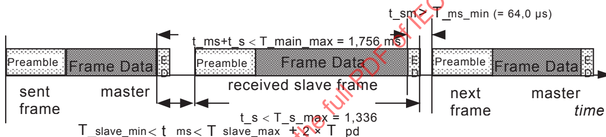
Figure 40 – Frame spacing measured at the master side
