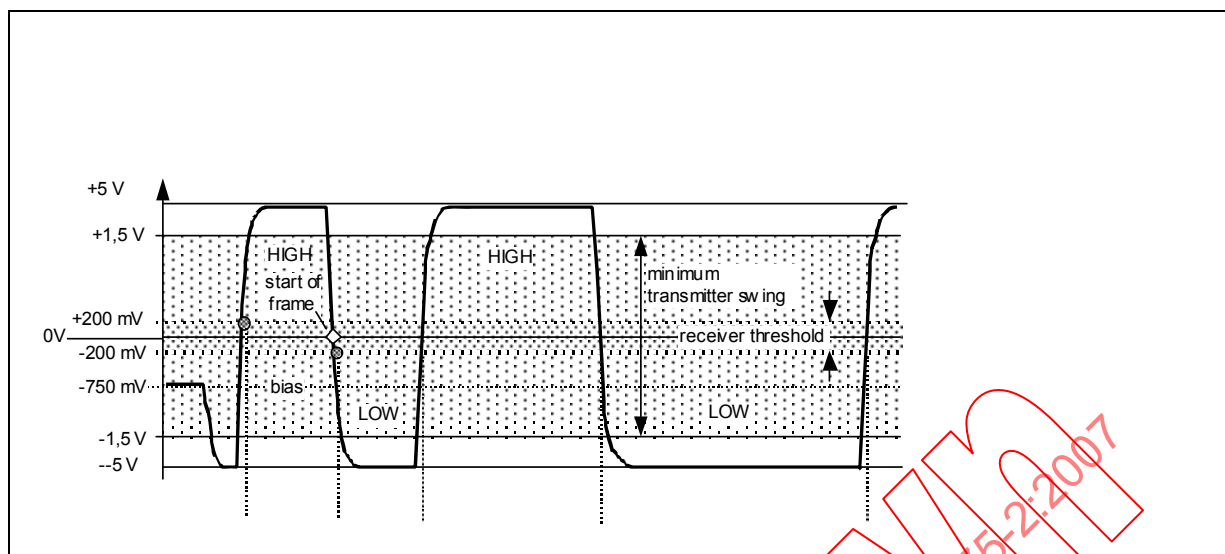
Figure 7 – Frame (ESD)
