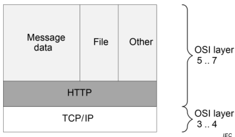
Figure 14 – Communication stacks
