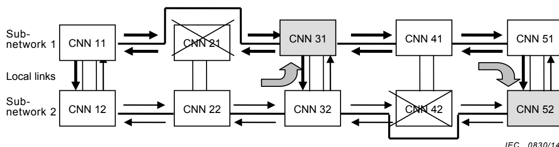
Figure D.27 – Re-configuration of transmission paths with double failures of CNNs over both sub-networks
