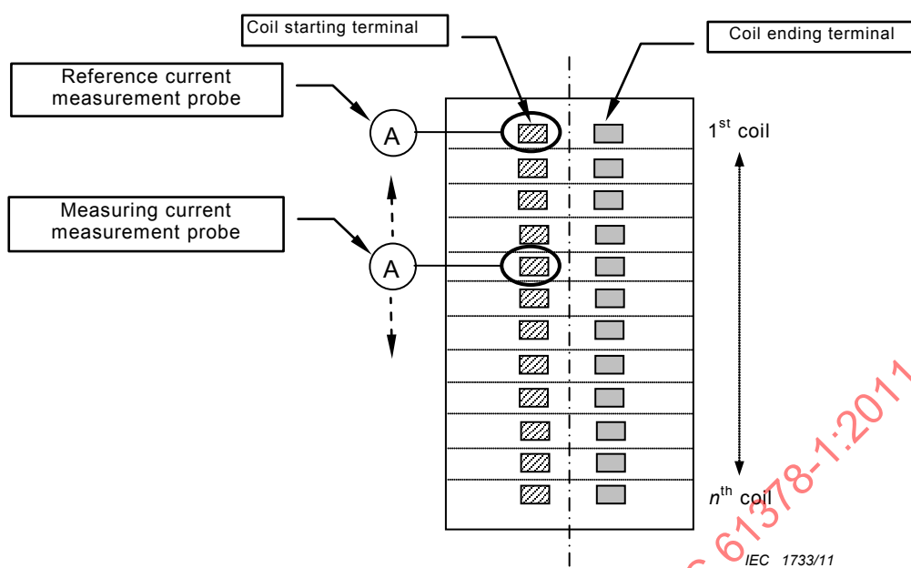
Figure C.1 – Example of valve high current winding and measurement equipment disposition
