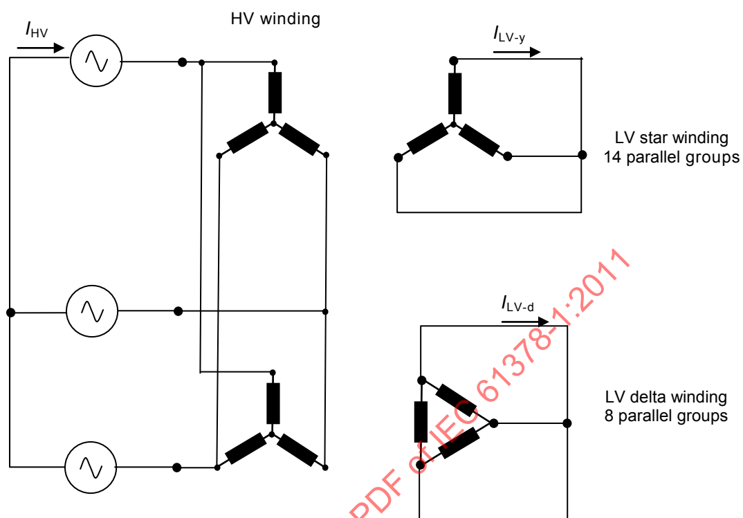
Figure C.3 – Measurement circuit for the in-phase measurement
