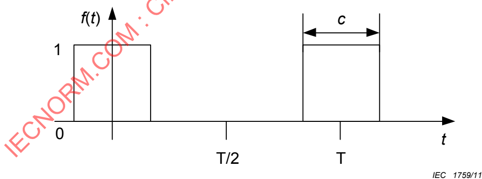
Figure J.2 – DSS Connection rectangular current blocks
