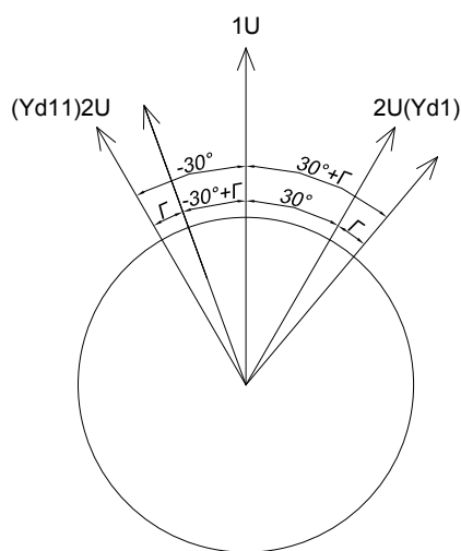
Figure I.4 – Example I.1 phase displacement
