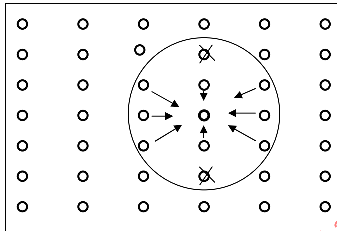
Figure D.1 – Configuration – Inside a wind farm with more than 2 rows
