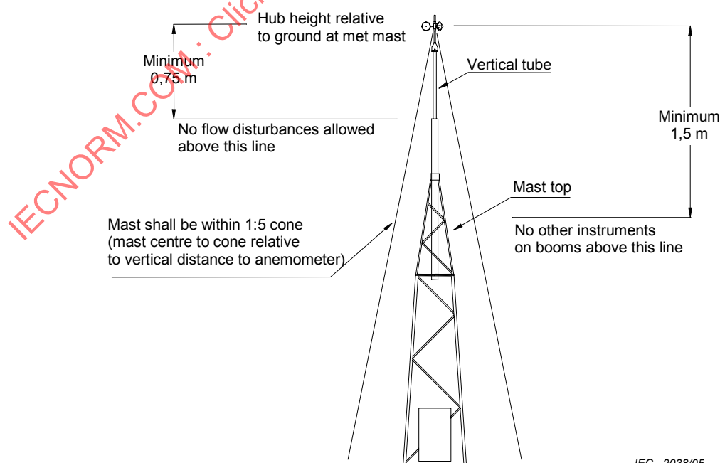
Figure G.1 – Example of a top-mounted anemometer and requirements for mounting
