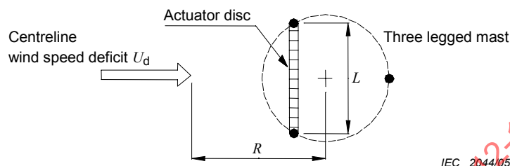
Figure G.7 – Representation of a three-legged lattice mast showing the centre-line wind speed deficit, the actuator disc representation of the mast with the leg distance L and distance R from the centre of the mast to the point of observation
