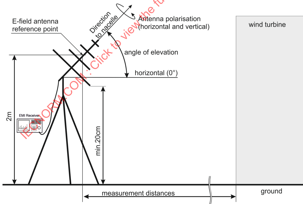
Fig. 3: Example of a test setup of a electric field strength measurement
