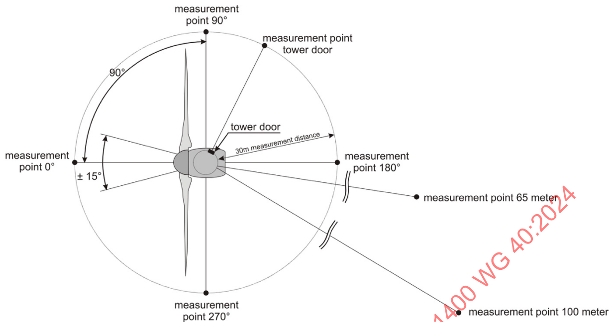
Fig. 4: Example of a test configuration for an EMC measurement on a wind turbine. Measurement points relative to the wind turbine hub.
