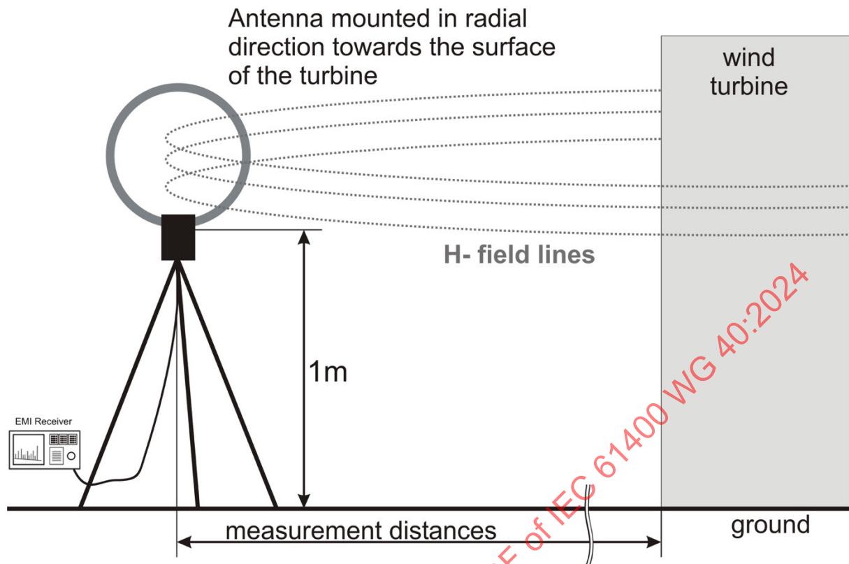
Fig. 2: Example of a test setup of a magnetic field strength measurement
