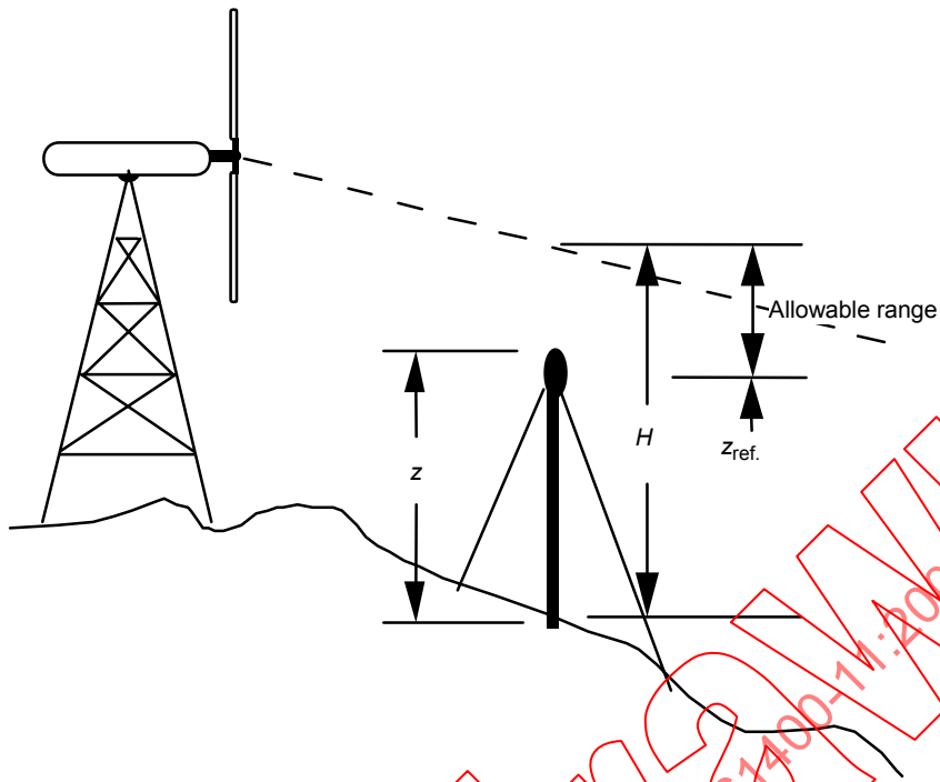
Figure 6 – Allowable range for anemometer height – cross section
