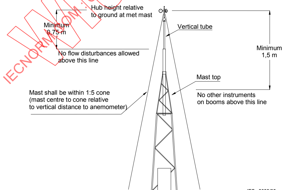
Figure G.1 – Example of a top-mounted anemometer and requirements for mounting
