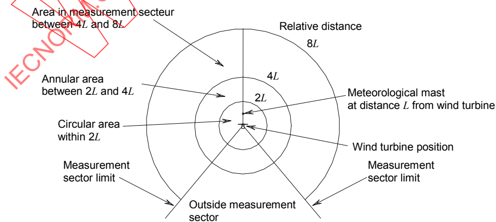
Figure B.1 – Illustration of area to be assessed, top view
