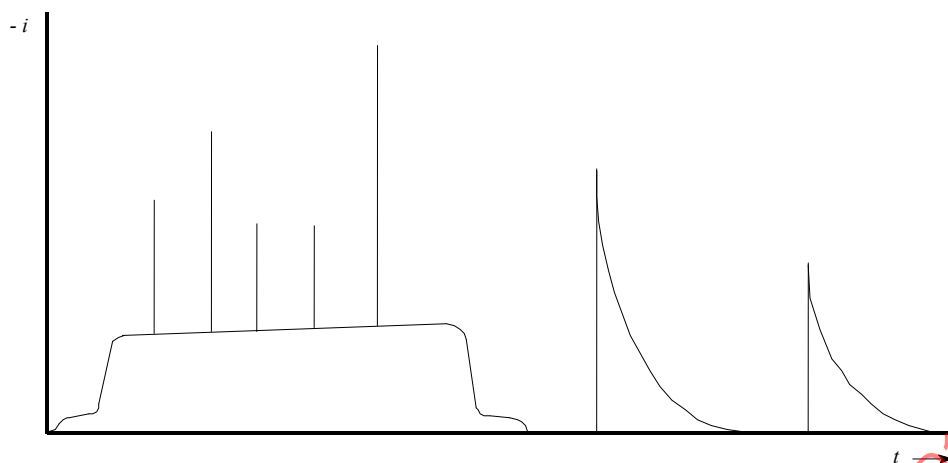
Figure A.8 – Typical profile of a negative upward initiated flash
