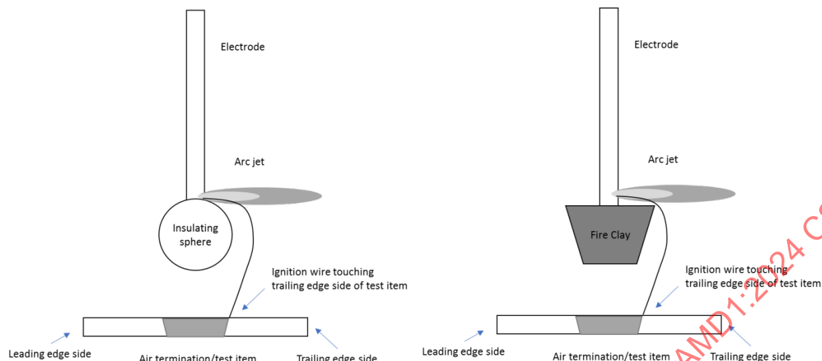
Figure D.13 – Typical jet diverting test electrodes
