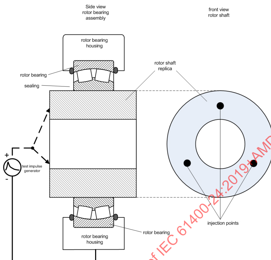
Figure P.3 – Possible test setup for a main bearing
