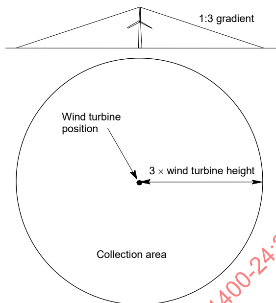
Figure 1 – Collection area of the wind turbine
