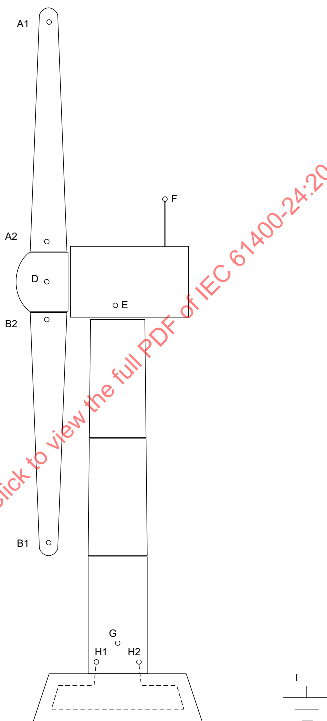
Figure J.1 – Example of measuring points
