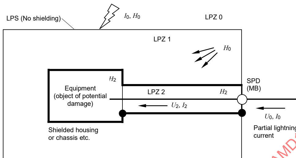
c) SPM using internal line shielding and SPD protection at entry of LPZ 1 – Equipment protected against conducted surges ( U_2 < U_0 and I_2 < I_0 ) and against radiated magnetic fields ( H_2 < H_0 )
