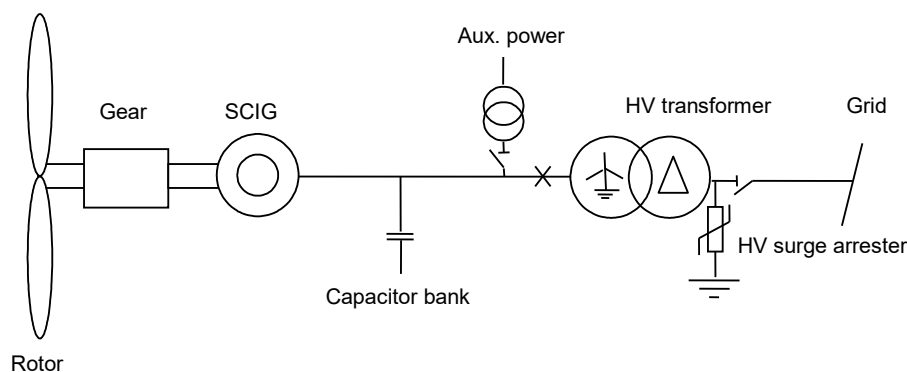
a) Squirrel cage induction generator (SCIG)
