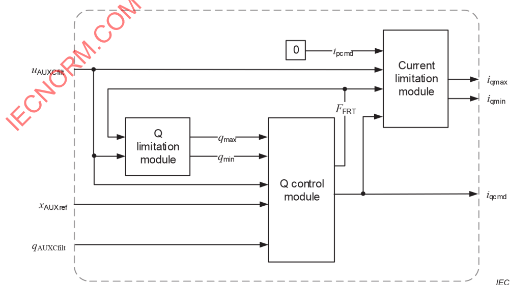
Figure 13 – Modular structure of the STATCOM control model
