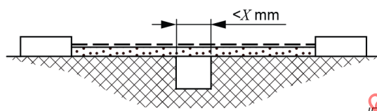
Figure F.1 a) – Measurement of ribs: examples
