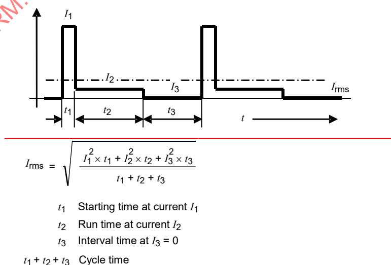
Figure E.6 — Example of average heating effect calculation
