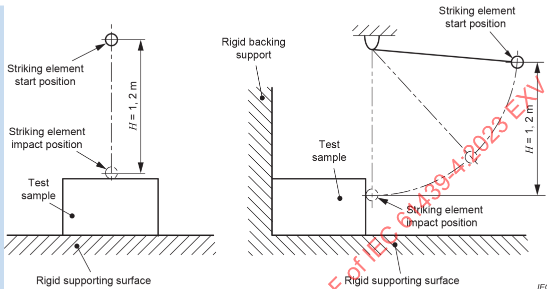
Figure 101 – Impact test using striking element
