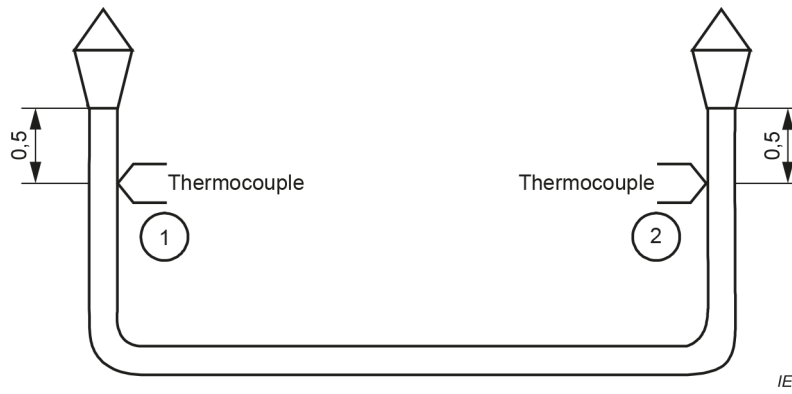
Figure 1 – Terminations tested in air
