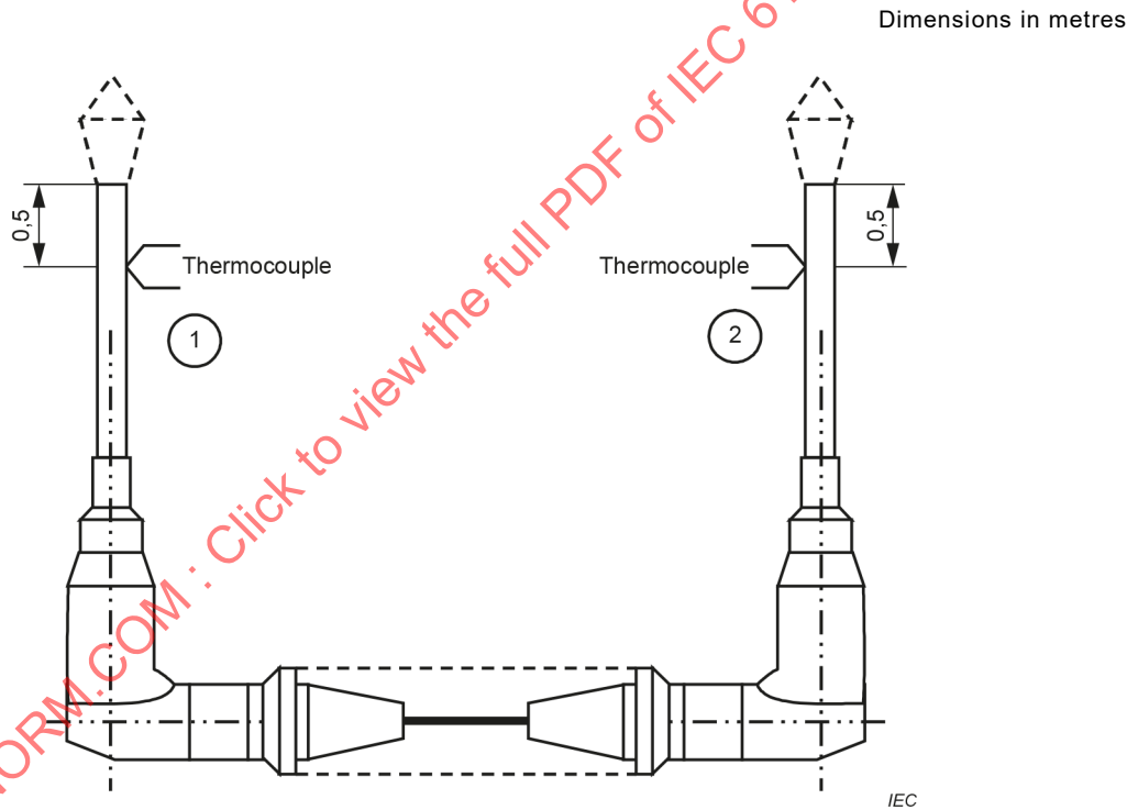
Figure 2 – Joints tested in air
