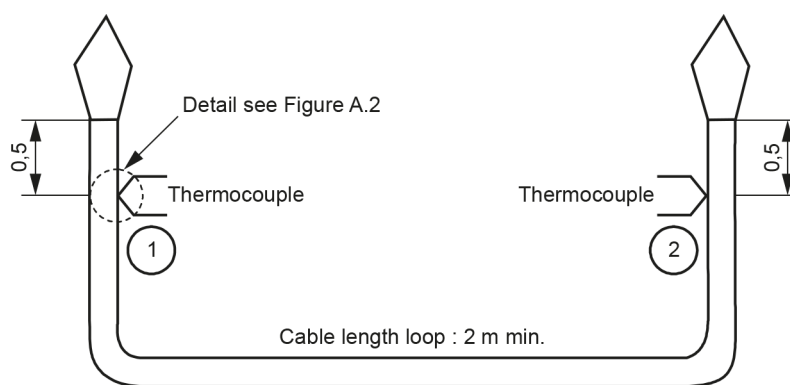
Figure A.1 – Reference cable
