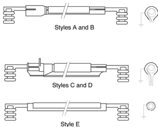
Figure 2 – Electrodes for proof-test A1
