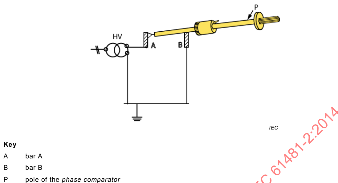
Figure 10 – Electrical connection of the bars
