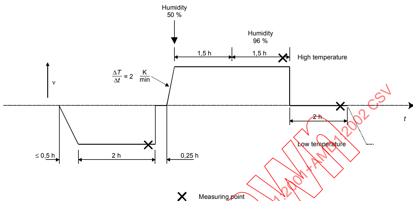
Figure 13 – Curve of test cycle for climatic resistance
