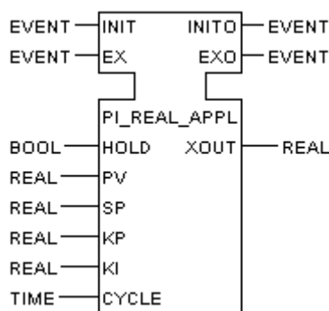
Figure 15a – External interface
