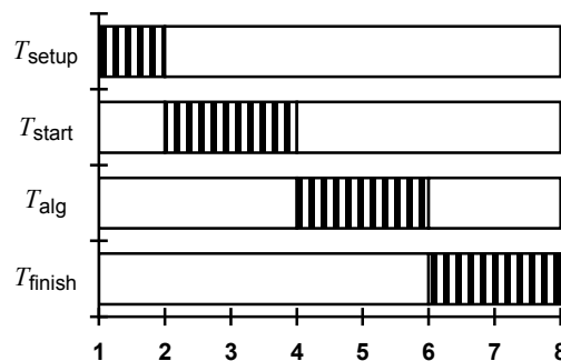
Figure 6 – Execution model
