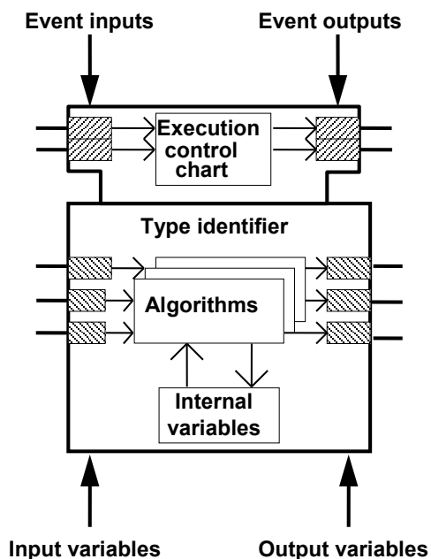
Figure 9a – Basic function block (5.2)
