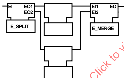
Figure A.1a – Explicit representation
