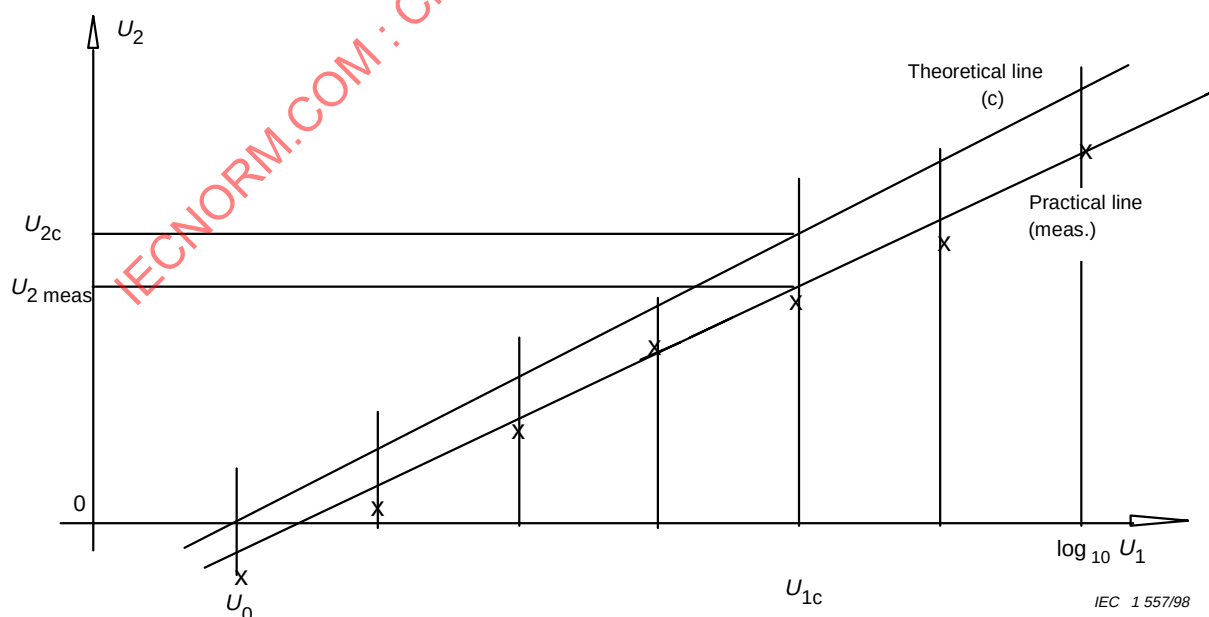
Figure 10 – Static error
