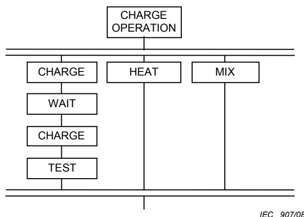
Figure 7 – Non-persistent process actions
