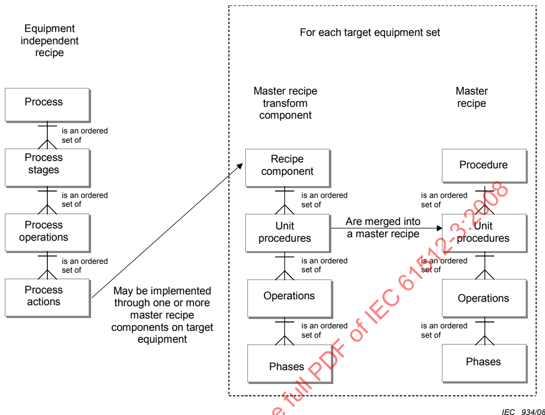
Figure 34 – Mapping of a process action to one or more unit procedures
