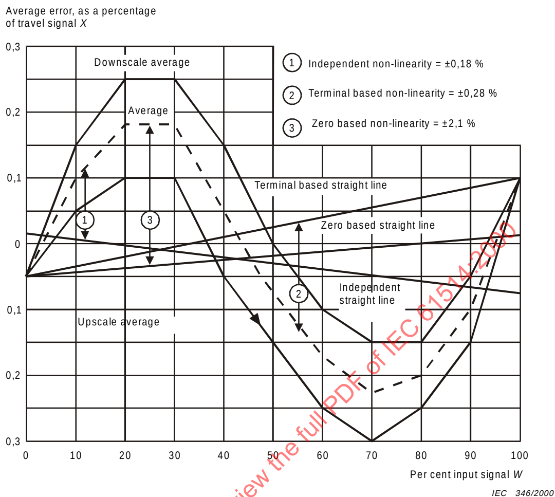
Figure 4 – Typical error plot
