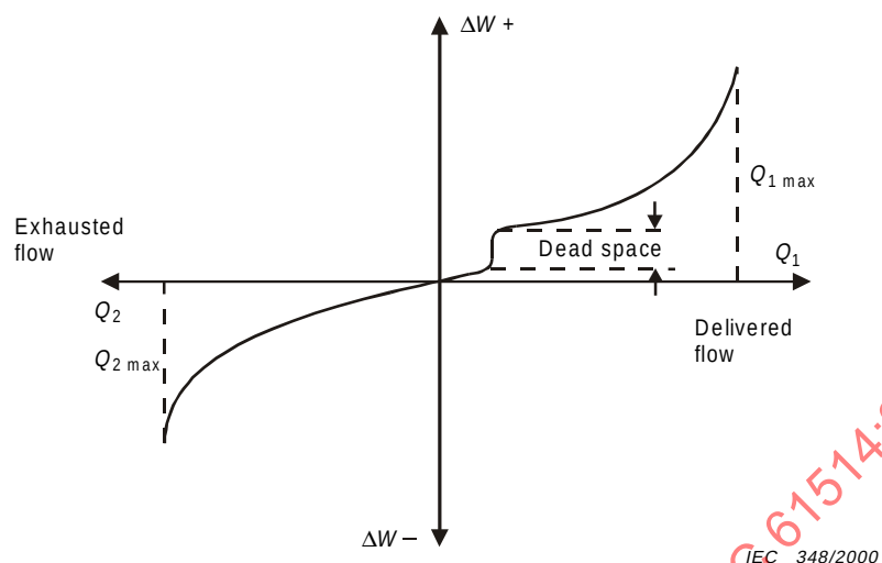
Figure 6 – Typical air flow characteristic
