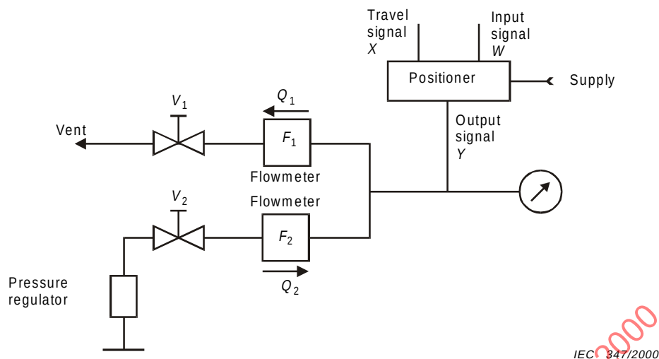
Figure 5 – Test arrangement for measurement of airflow characteristic
