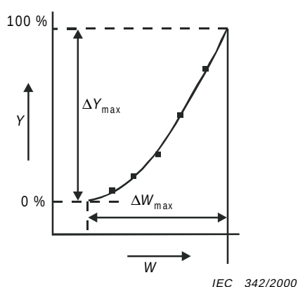
Figure 2a – Single-acting positioner
