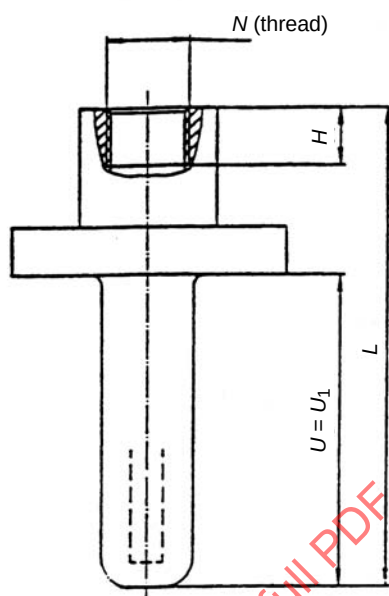
Figure 5 – Type C – External configuration
