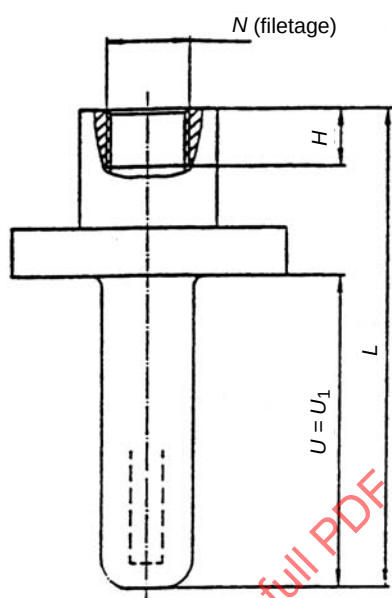
Figure 5 – Type C – Configuration extérieure
