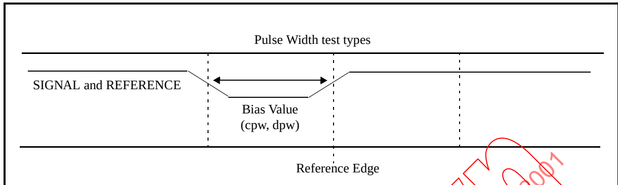
Figure 8-10 Different edges
