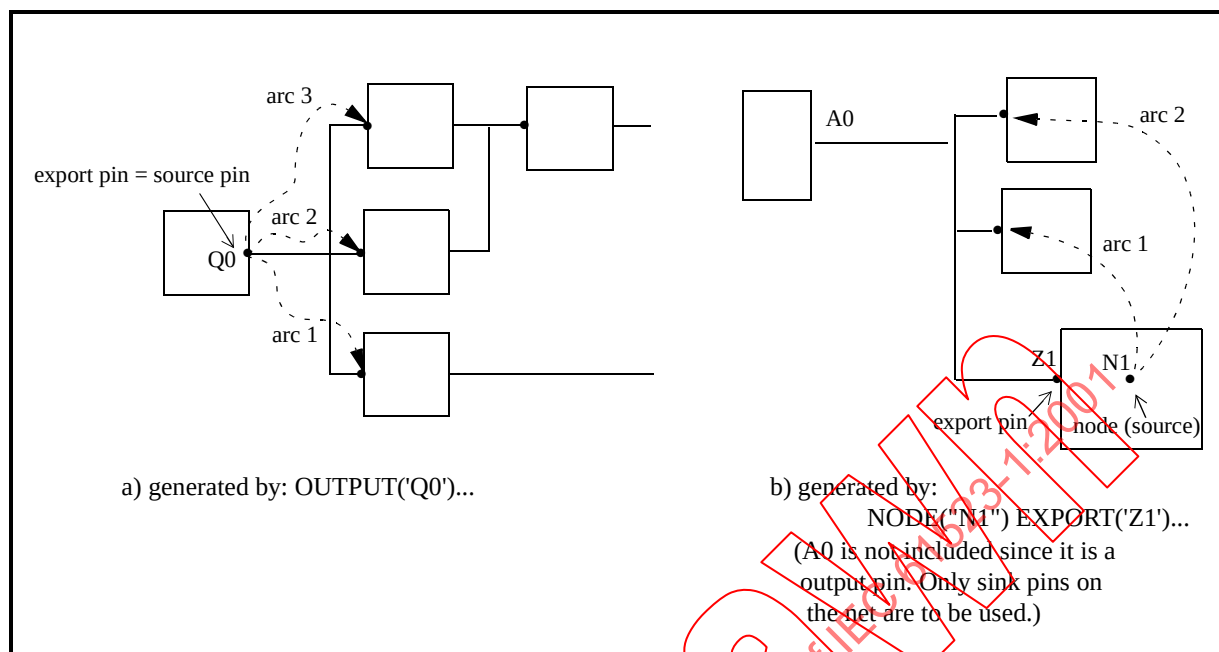
Figure 8-12 Additional MODELPROC results
