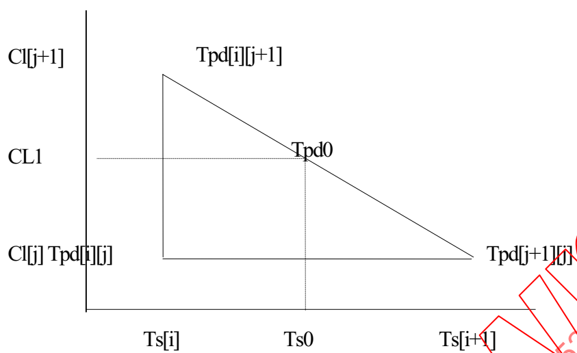
Figure 6. Interpolation for right angle triangle
