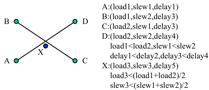
Figure C.5 Position relation of each point (a plane)
