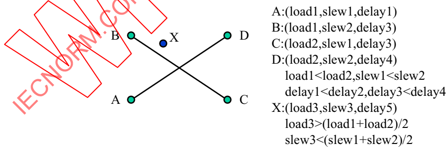
Figure C.3 Relation of each point
