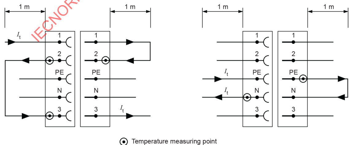
Figure B.2 – 3P + N + PE installation couplers, 3 phases loaded (left figure), N and PE loaded (right figure)
