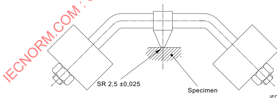
Figure 14 – Ball-pressure apparatus
