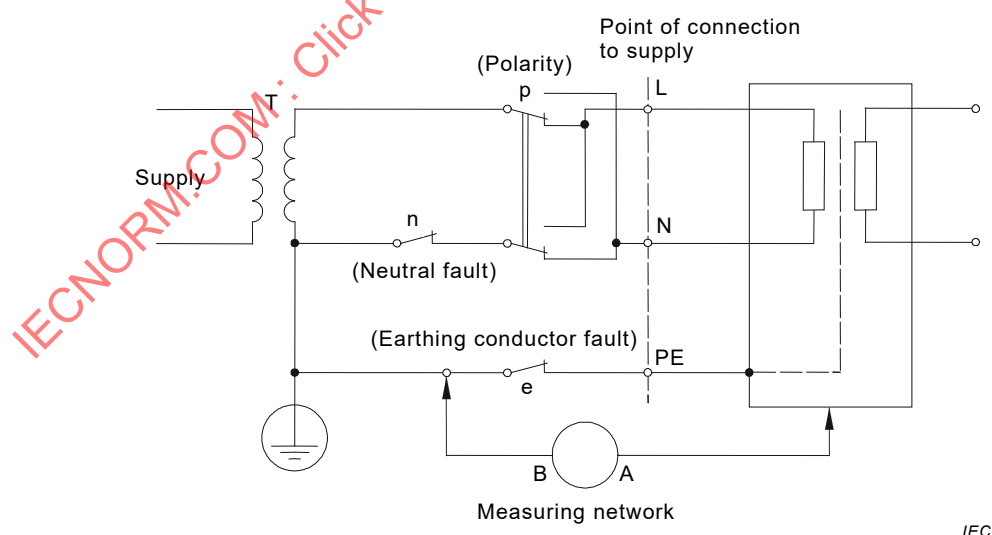
Figure 10 – Test configuration: single-phase equipment on star TN or TT system
