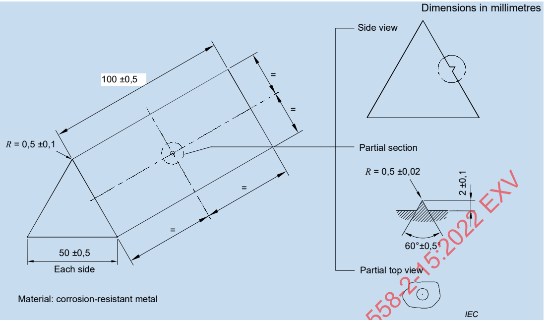
Figure 13a – Mandrel
