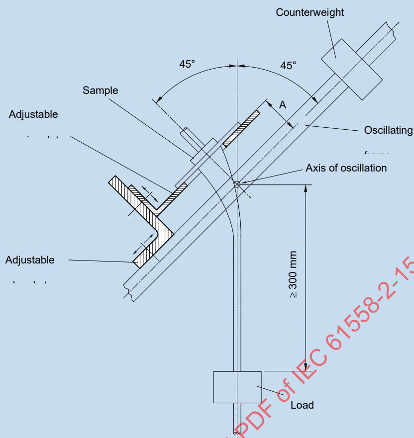
Figure 104 – Flexing test apparatus
