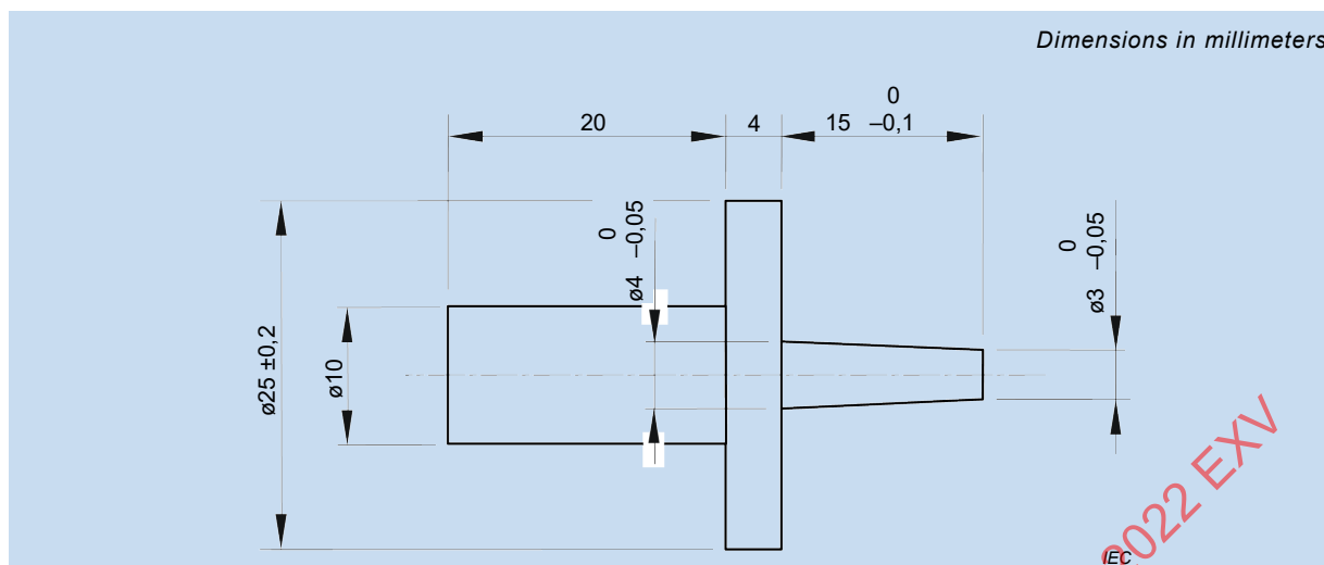
Figure 2 – Test pin (see IEC 61032, test probe 13)
