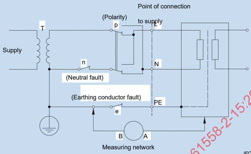
Figure 9 – Test configuration: single-phase equipment on star TN or TT system
