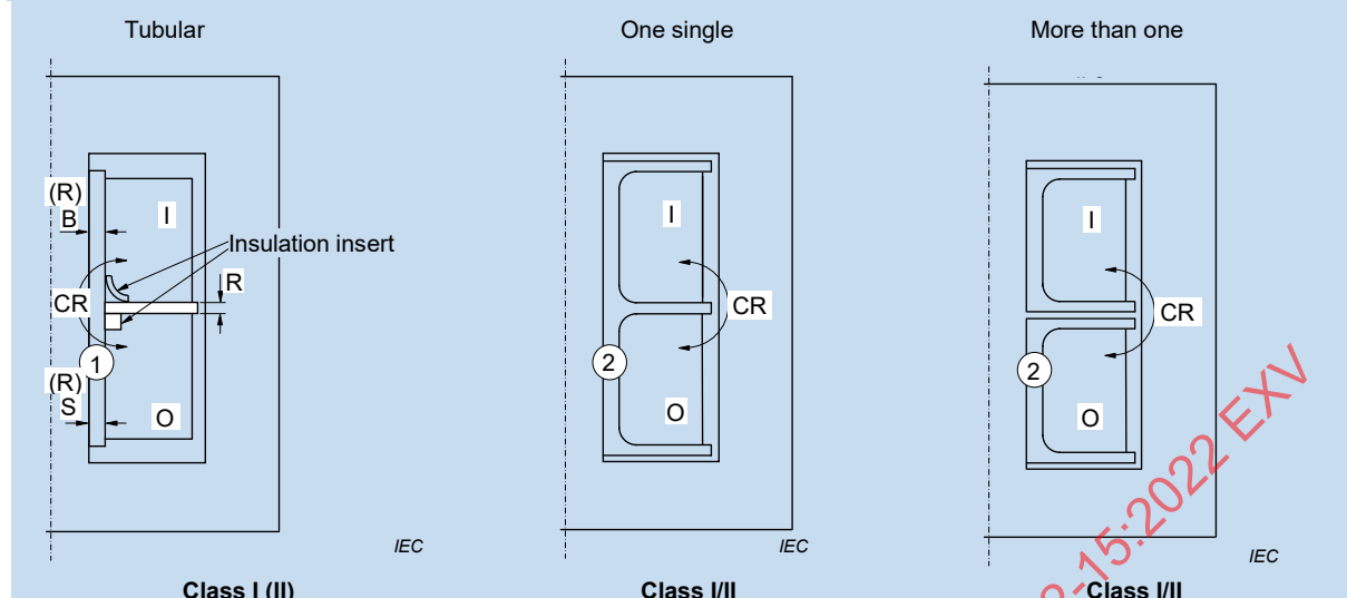
Figure M.2 – Examples for side-by-side type constructions
