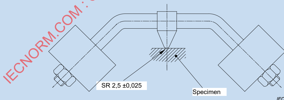
Figure 106 – Ball-pressure apparatus
