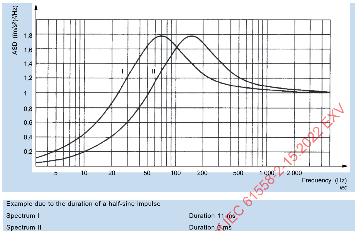
Figure 7 – Normalised spectrum of shock
