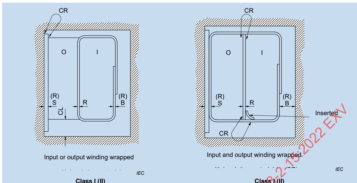
Figure M.4 – Examples for wrapped winding constructions
