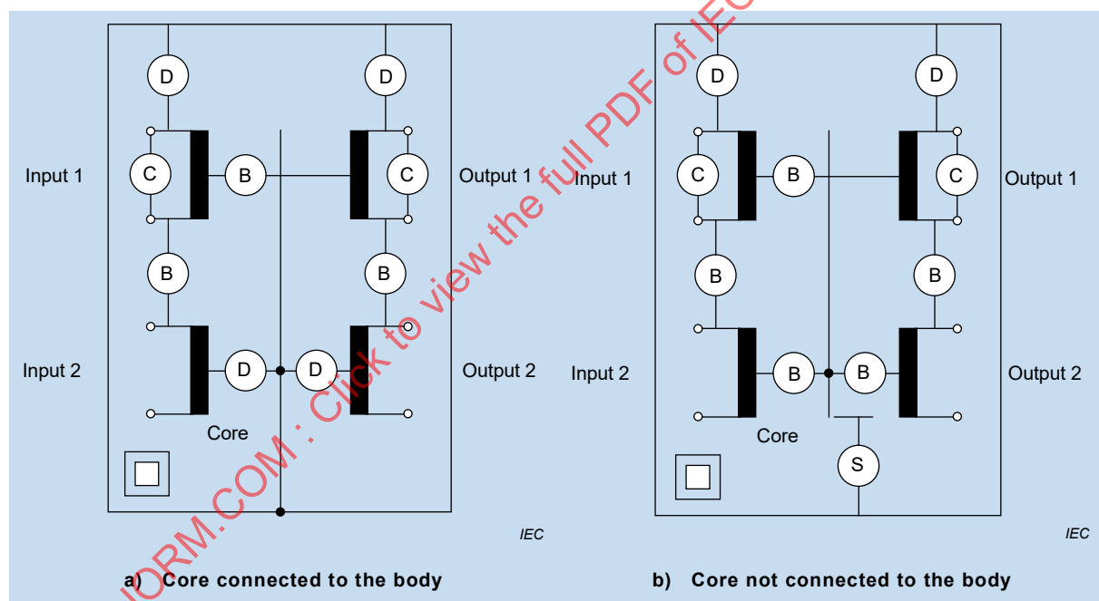
Figure P.3 – Transformer of class II construction with metal enclosure
