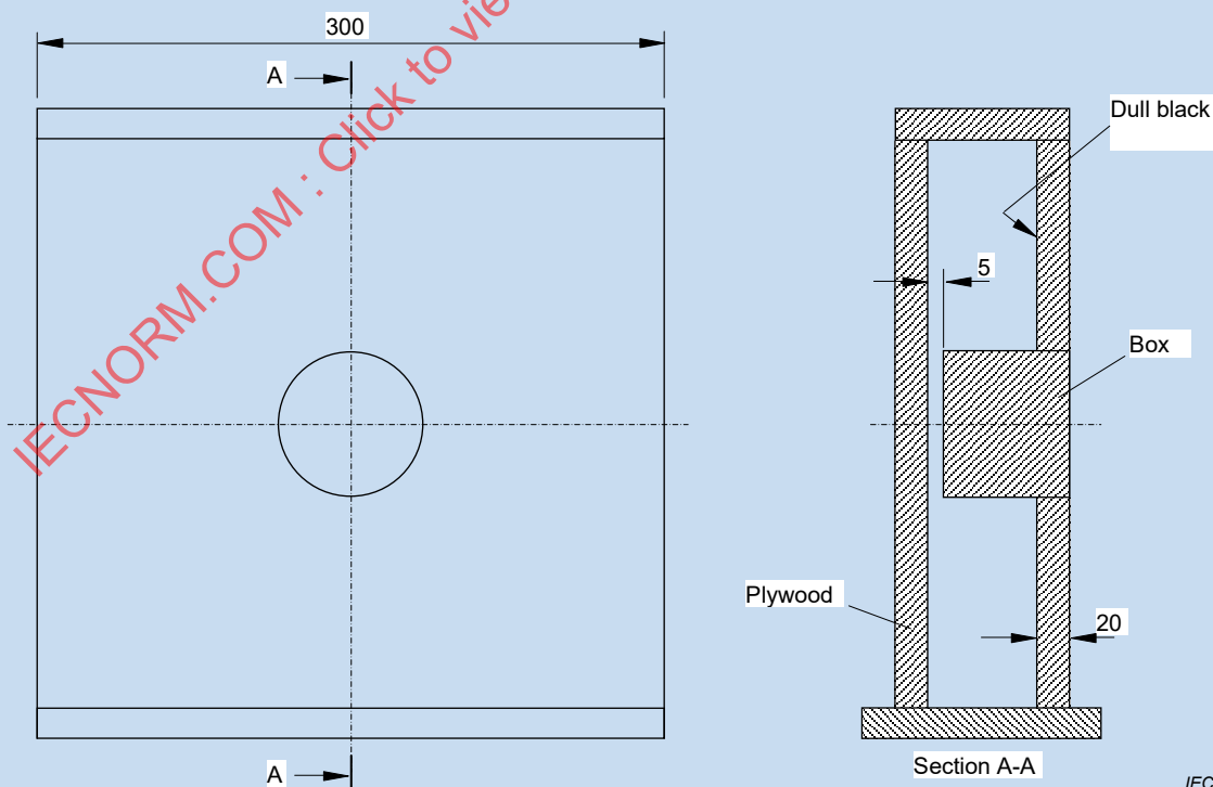
Figure 1 – Mounting box for flush-type transformer
