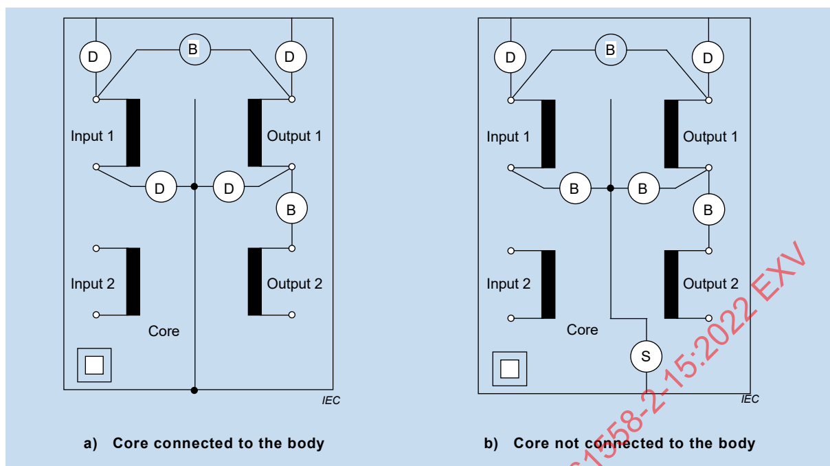
Figure N.2 – Transformer of class II construction with metal enclosure
