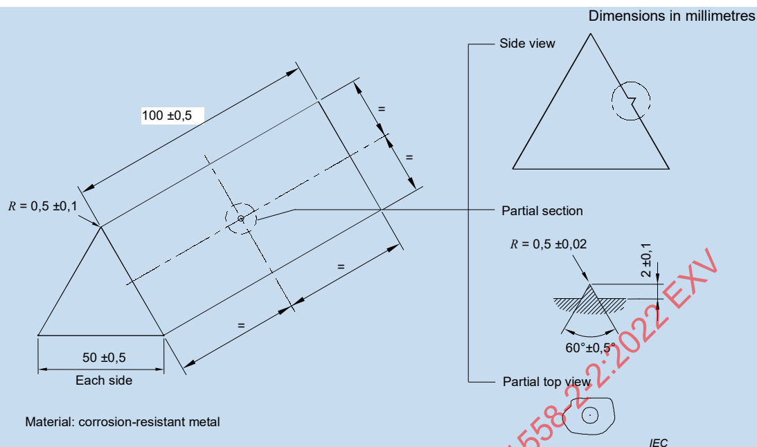
Figure 13a – Mandrel
