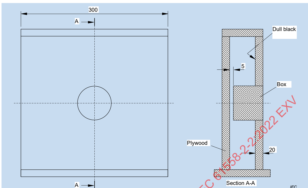
Figure 2 – Mounting box for flush-type transformer
