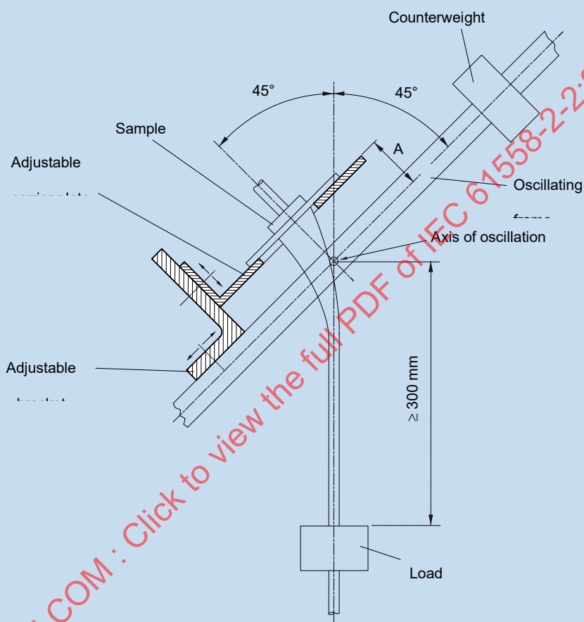
Figure 12 – Flexing test apparatus
