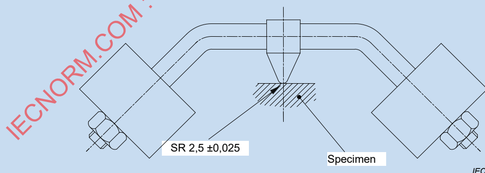
Figure 14 – Ball-pressure apparatus
