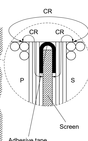
Adhesive tape
