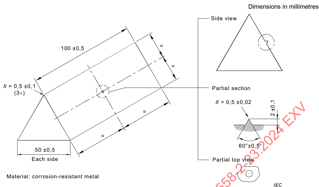
Figure 13a – Mandrel
