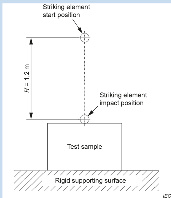
Figure 101 – Impact test for horizontal surface
