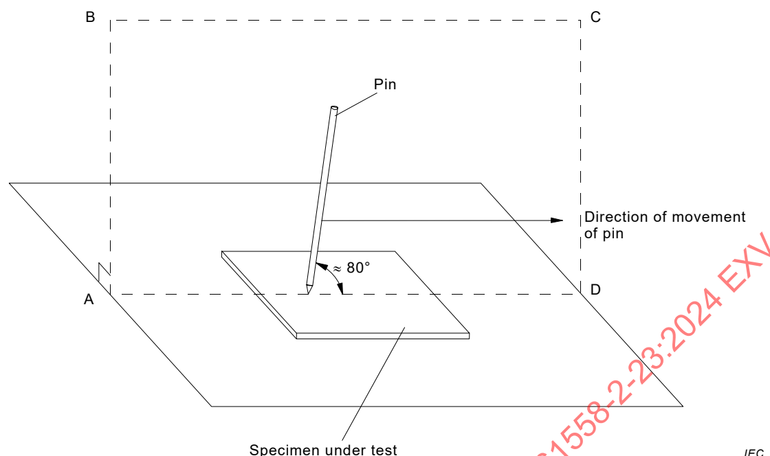
Figure 11 – Abrasion resistance test for insulating coated layers
