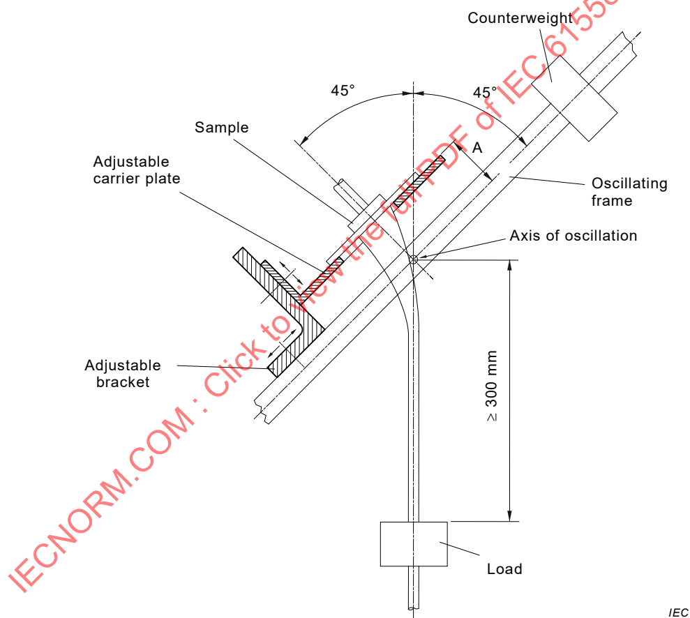
Figure 12 – Flexing test apparatus
