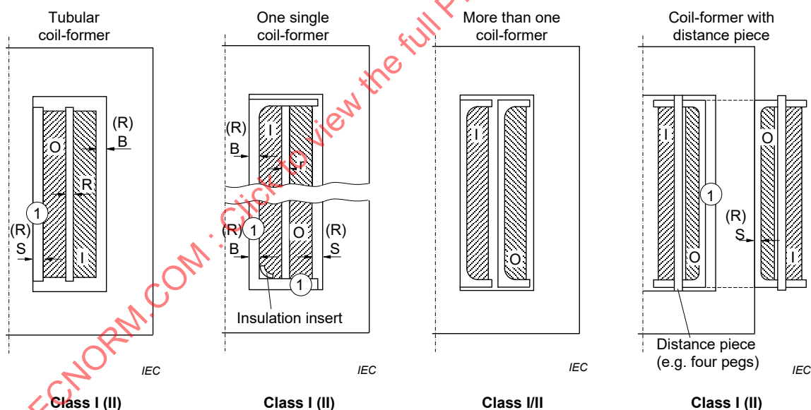
Figure M.1 – Examples for concentric type constructions
